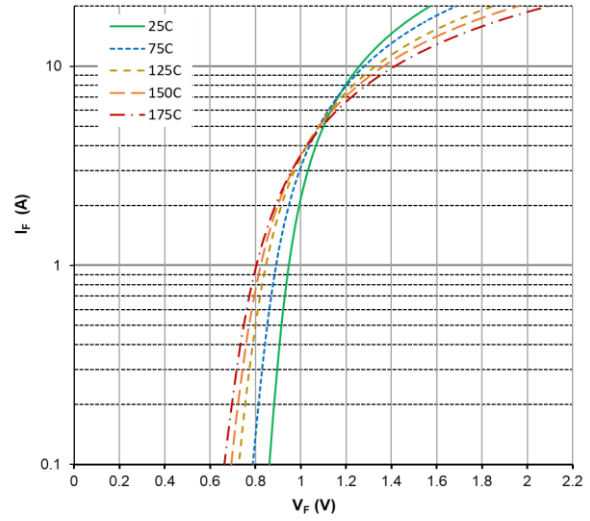
Figure 2. Forward Characteristics
