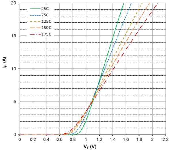
Figure 1. Forward Characteristics
